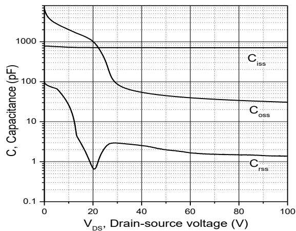
Figure 3. Typ. capacitances
