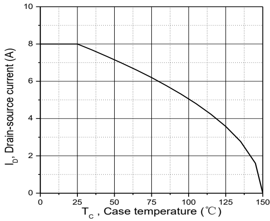
Figure 9. Drain current
