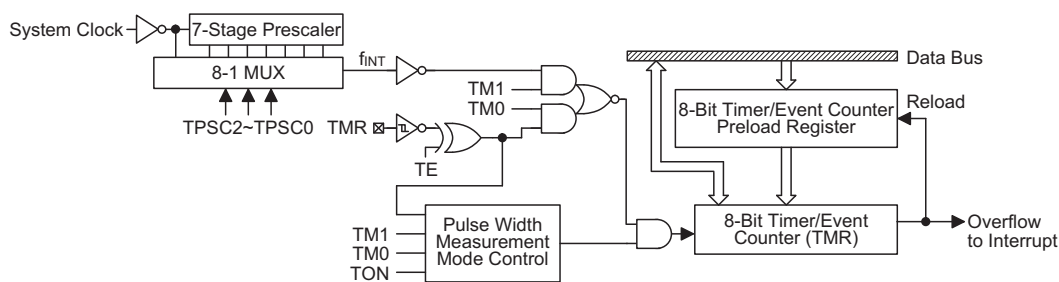
Timer/Event Counter
