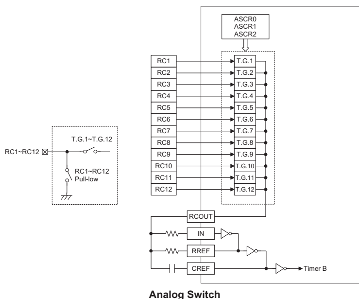
Analog Switch
