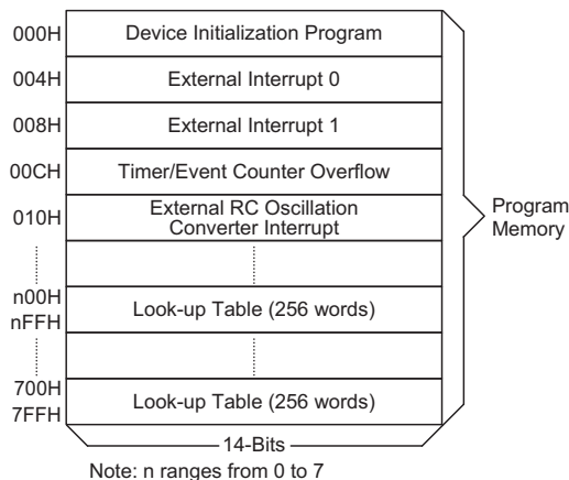
Program Memory
