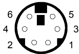
PS2 Mouse (6-pin female)
